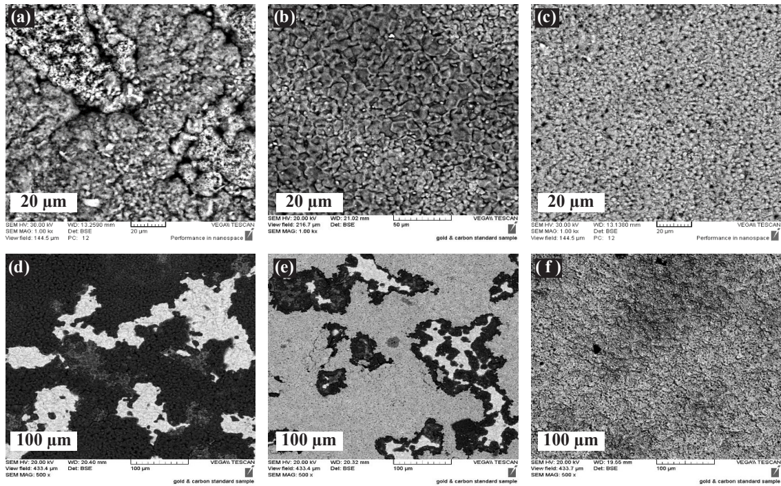
Fig. 10. SEM surface observations of the coating prior to the oxidation tests (a) AHHZ0 (b) AHHZ10 (c) AHHZ30 and the microstructure after the oxidation tests at 1000 °C for 120 hours (d) AHHZ0 (e) AHHZ10 and (f) AHHZ30.
