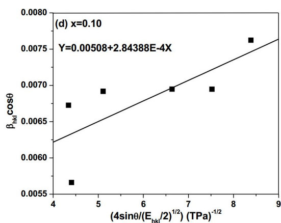
Figure 6(a-d). The plots \beta_{hkl}\cos\theta Vs 4\sin\theta(2/E_{hkl})^{1/2} of \text{Zn}_{1-x}\text{Mn}_x\text{O}
