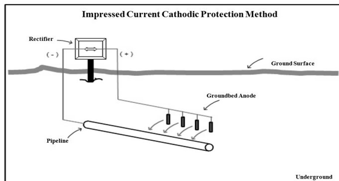
Fig. 1. ICCP Method
