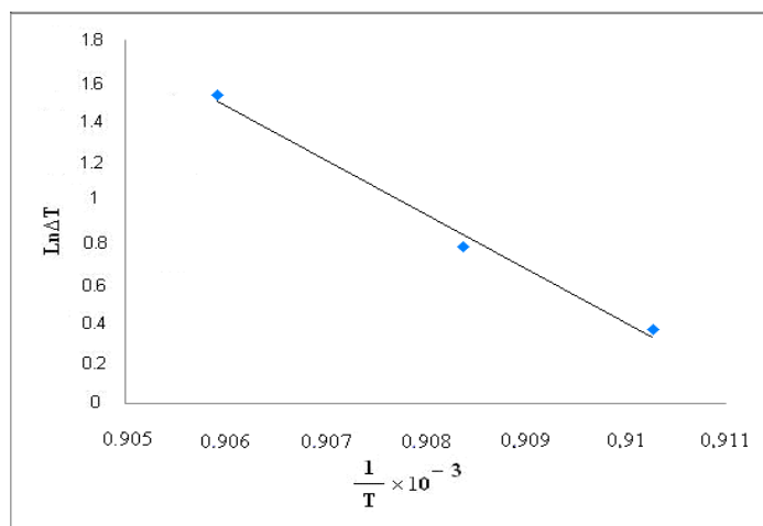
Fig 9. Variation of \ln \Delta T vs 1/T in \text{ST}_3\text{Z}_1\text{Y}_1 for determination of the Avrami exponent according to Marotta method
