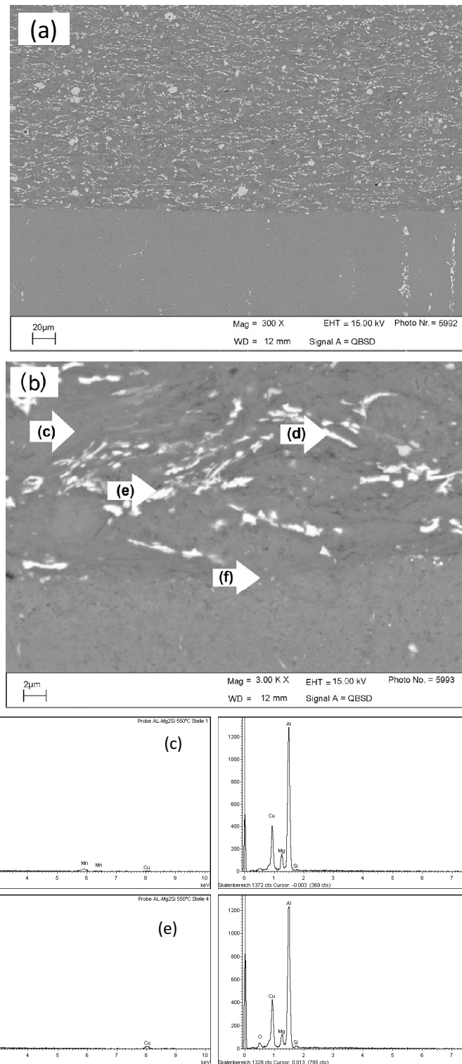
Fig. 6. Cross-sectional SEM micrographs of the clad layer obtained from SPS of MAed powder at 550 °C, a) clad layer b) clad layer-substrate interface, c-f) EDS microanalysis of selected points.
